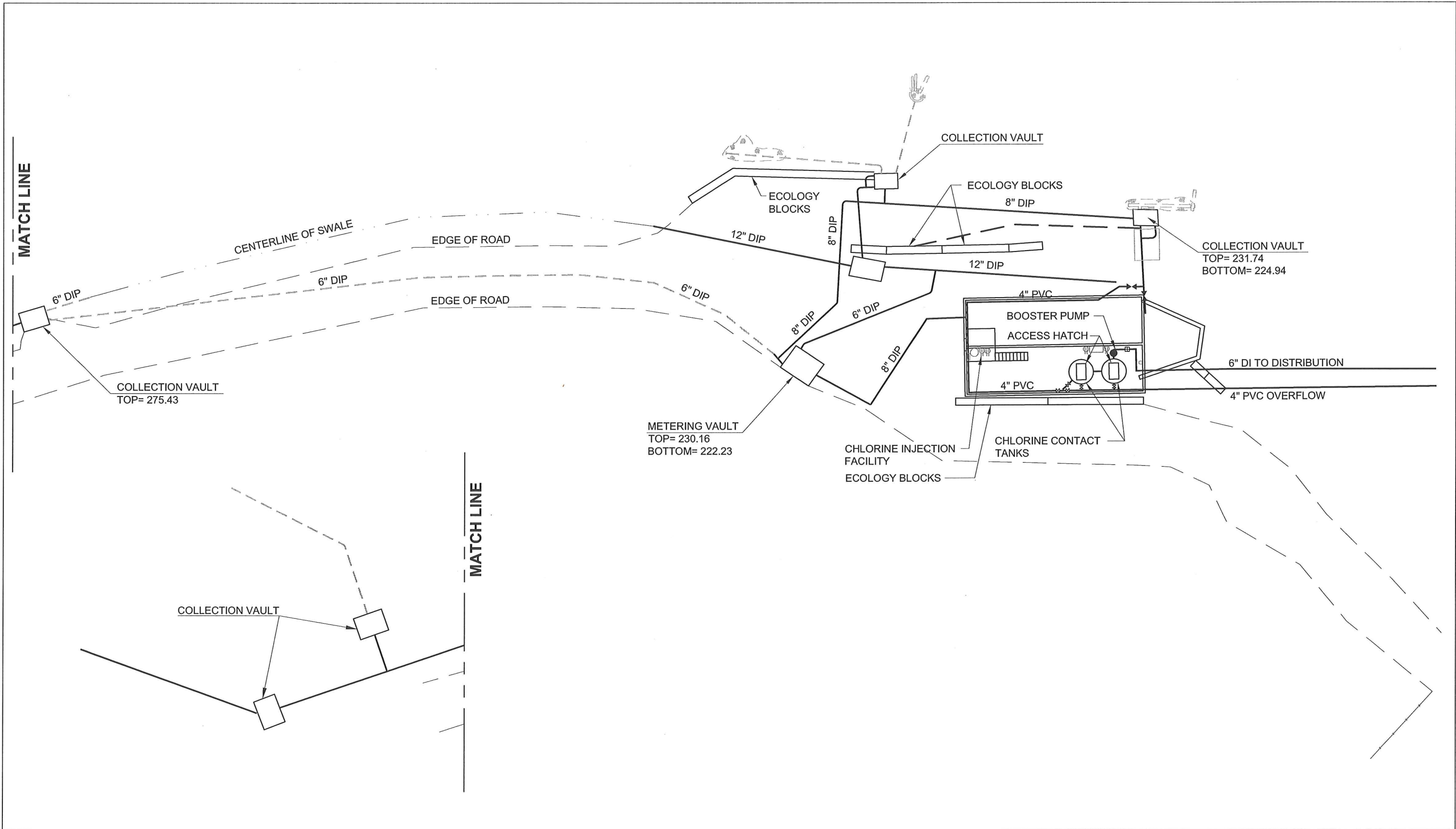
Figure 4-8 Summer Water System Elhi Springs
